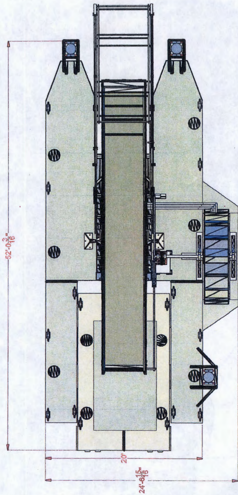
Harris Creek Trash Wheel Plan View
