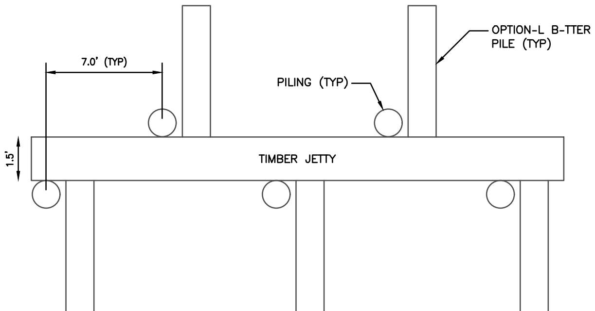
TIMBER JETTY DETAIL NOT TO SC-LE
