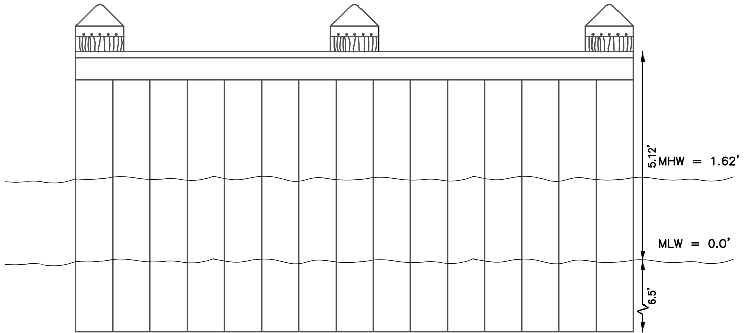
TIMBER JETTY DETAIL NOT TO SC-LE
