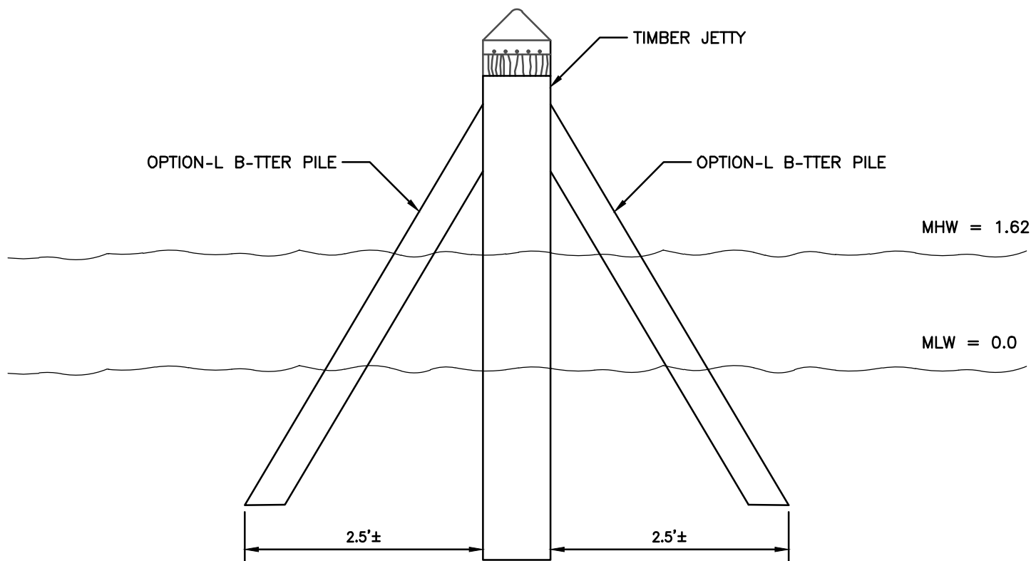
TIMBER JETTY DETAIL NOT TO SC-LE
