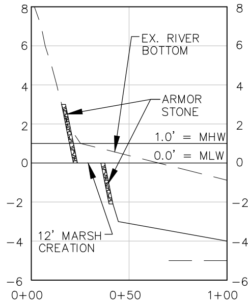
SECTION 'E-E'
