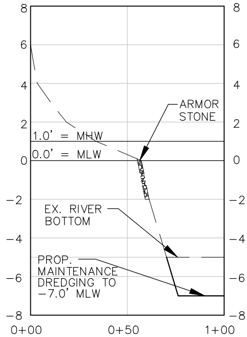
SECTION 'D-D'
