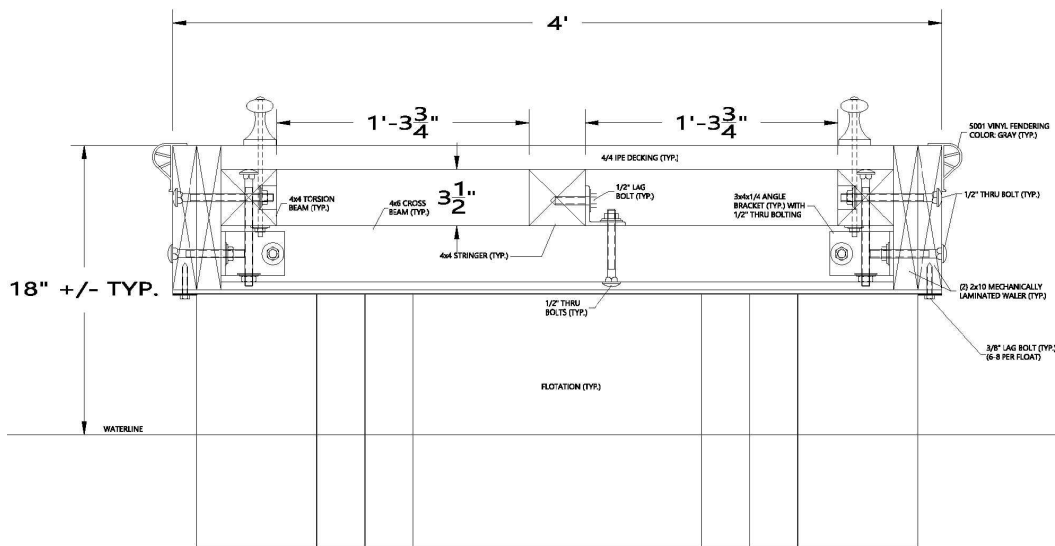
4' CROSS SECTION
