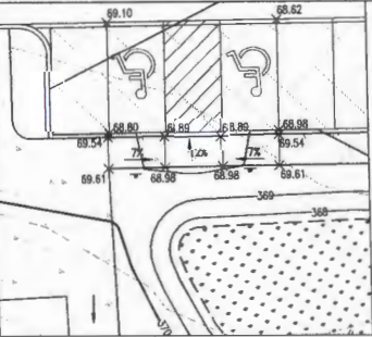
HANDICAP RAMP ENLARGED PLAN SCALE: 1"=10'
