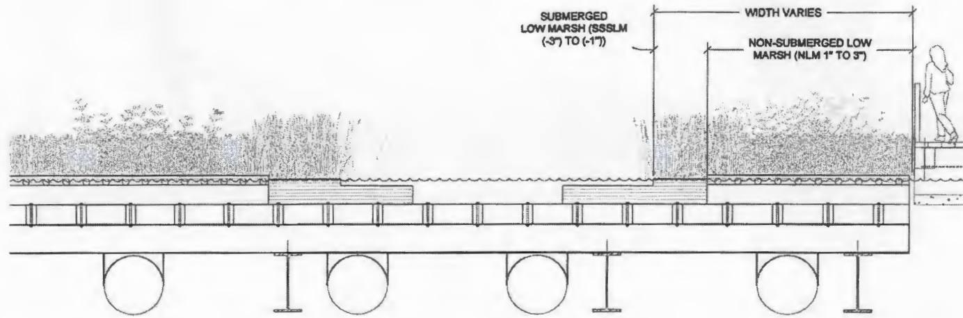
1 PLANTING ZONATION - STRUCTURED FLOATING WETLAND REPRESENTATIVE CROSS SECTION
